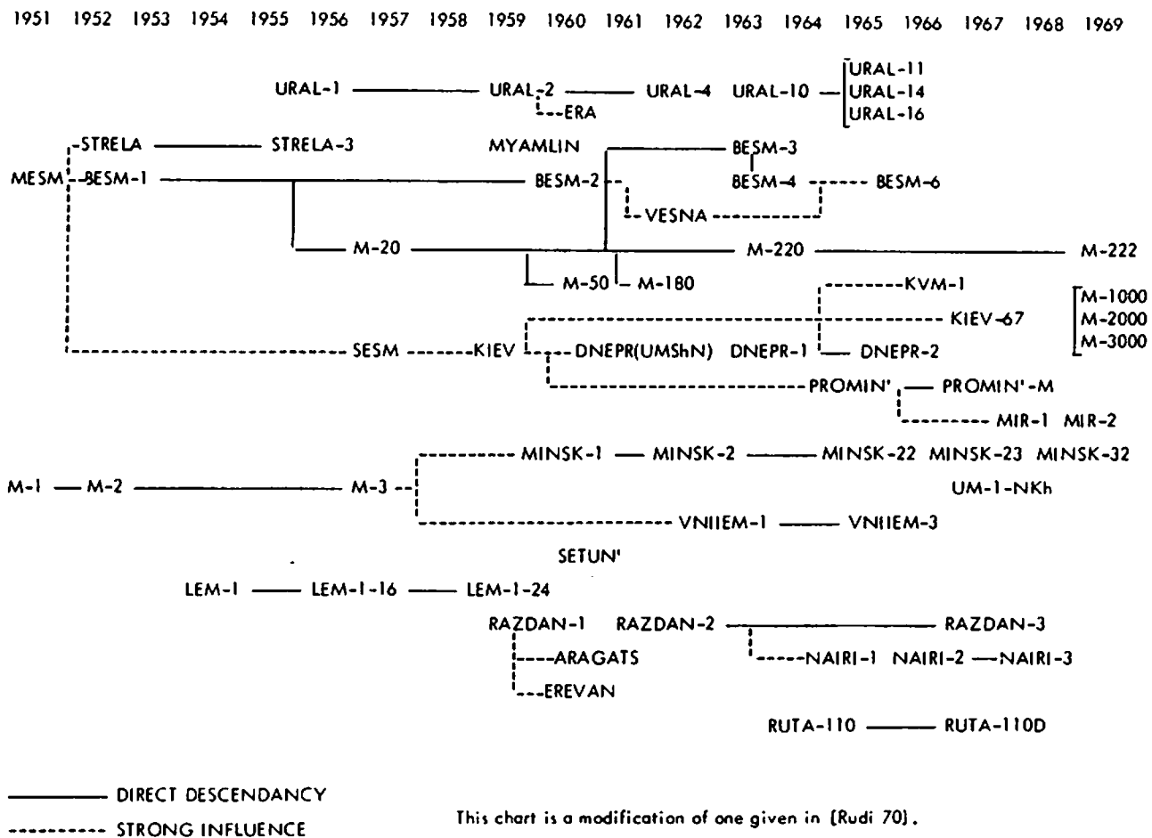
FIGURE 1. Soviet computers: 1951-1969.
